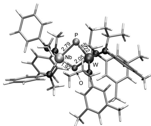
Figure 2. Optimized structure of model intermediate [\{\text{Ph(Me)N}\}_3\text{Nb}(\mu\text{-O})(\mu\text{-P})\text{W}\{\text{N}(i\text{Pr})\text{Ar}\}_3] . Selected bond lengths shown in Å.
